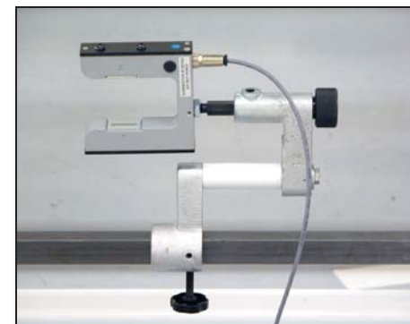
AUTOMATIC EDGE GUIDE Shown in this photo is the automatic edge guide with a pneumohydraulic controller.
